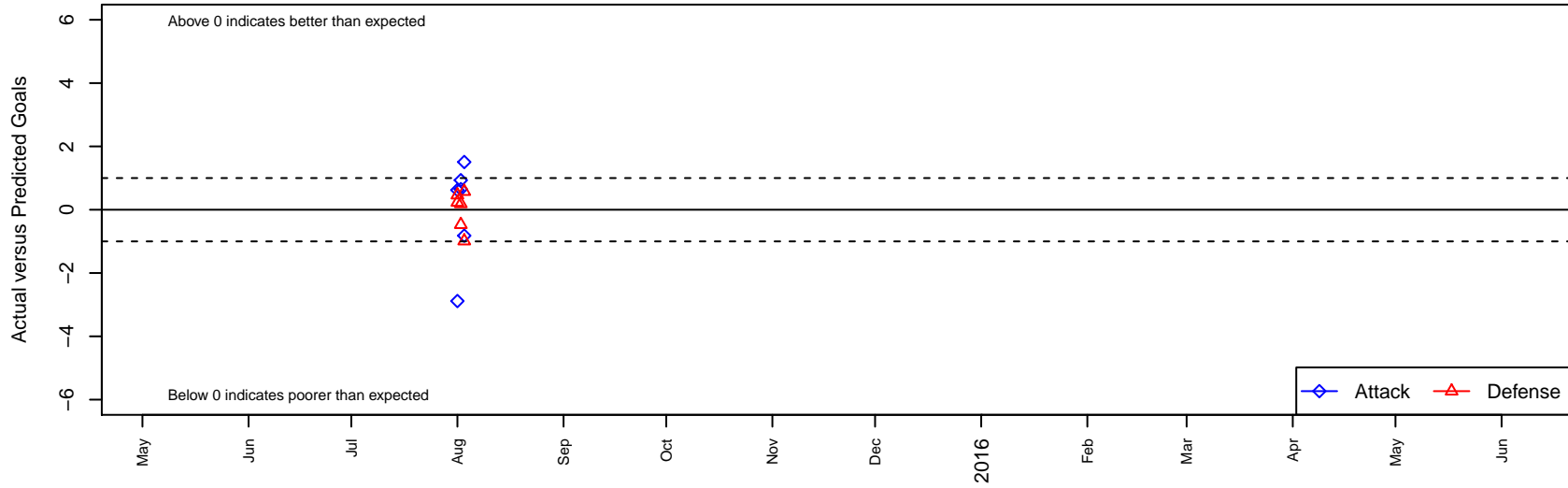
San Jose Earthquakes PDA 2003B Dots are actual minus expected GF (blue circles) and GA (red triangles). Blue line is smoothed change in attack strength. Red is smoothed change in defense strength.
